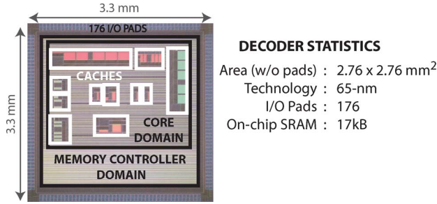
Fig. 19. Die photo of H.264/AVC baseline video decoder.
