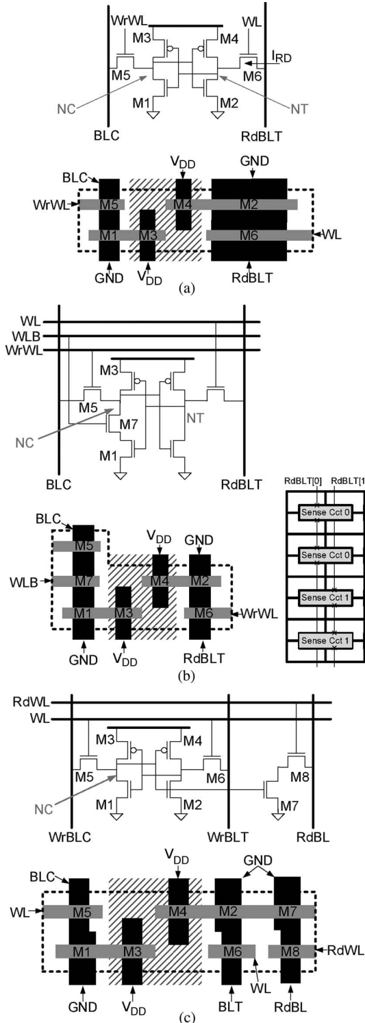
Fig. 7. Ultradynamic bit-cells utilizing: (a) 6T topology [48], (b) 7T topology [47], and (c) 8T topology [49].
