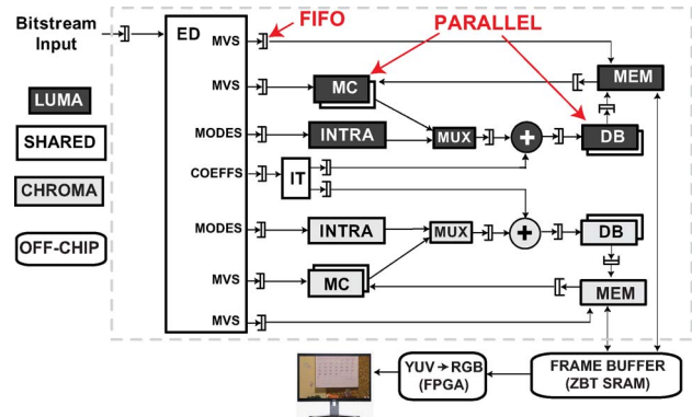
Fig. 16. H.264/AVC decoder architecture.
