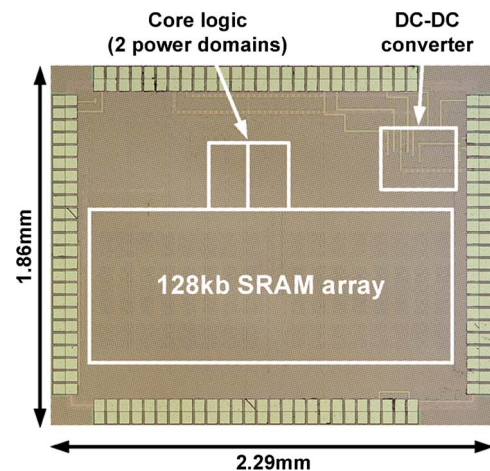
Fig. 21. Die micrograph of microcontroller test-chip.
